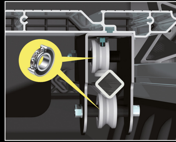
The working table is very strong and steady. • It slides on 2 steel square rails with 6 wheels; 4 over and 2 under. • Every wheel has 2 ball bearings for a total of 12.
